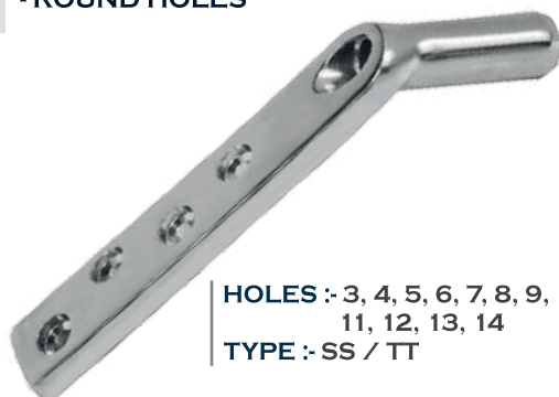
4.5 MM 130° DHS PLATE LONG BARREL - ROUND HOLES
